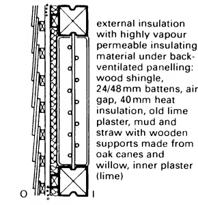
7 Exterior panelling
